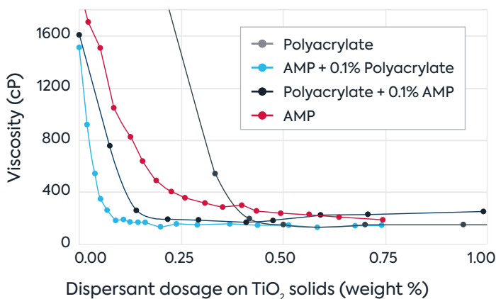
Dispersant Demand Curve
