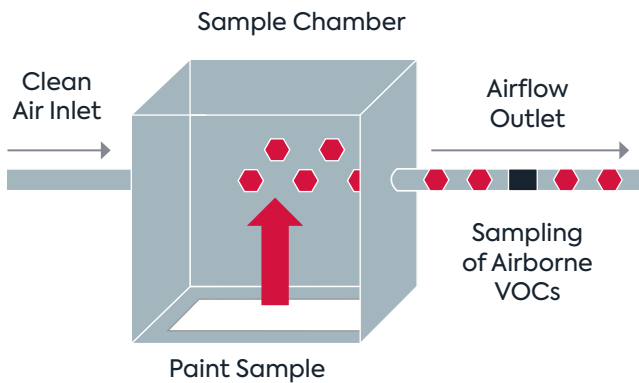
Schematic of a small-scale emissions testing chamber.
